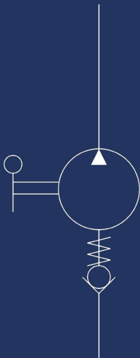
HYDRAULIC DIAGRAM
